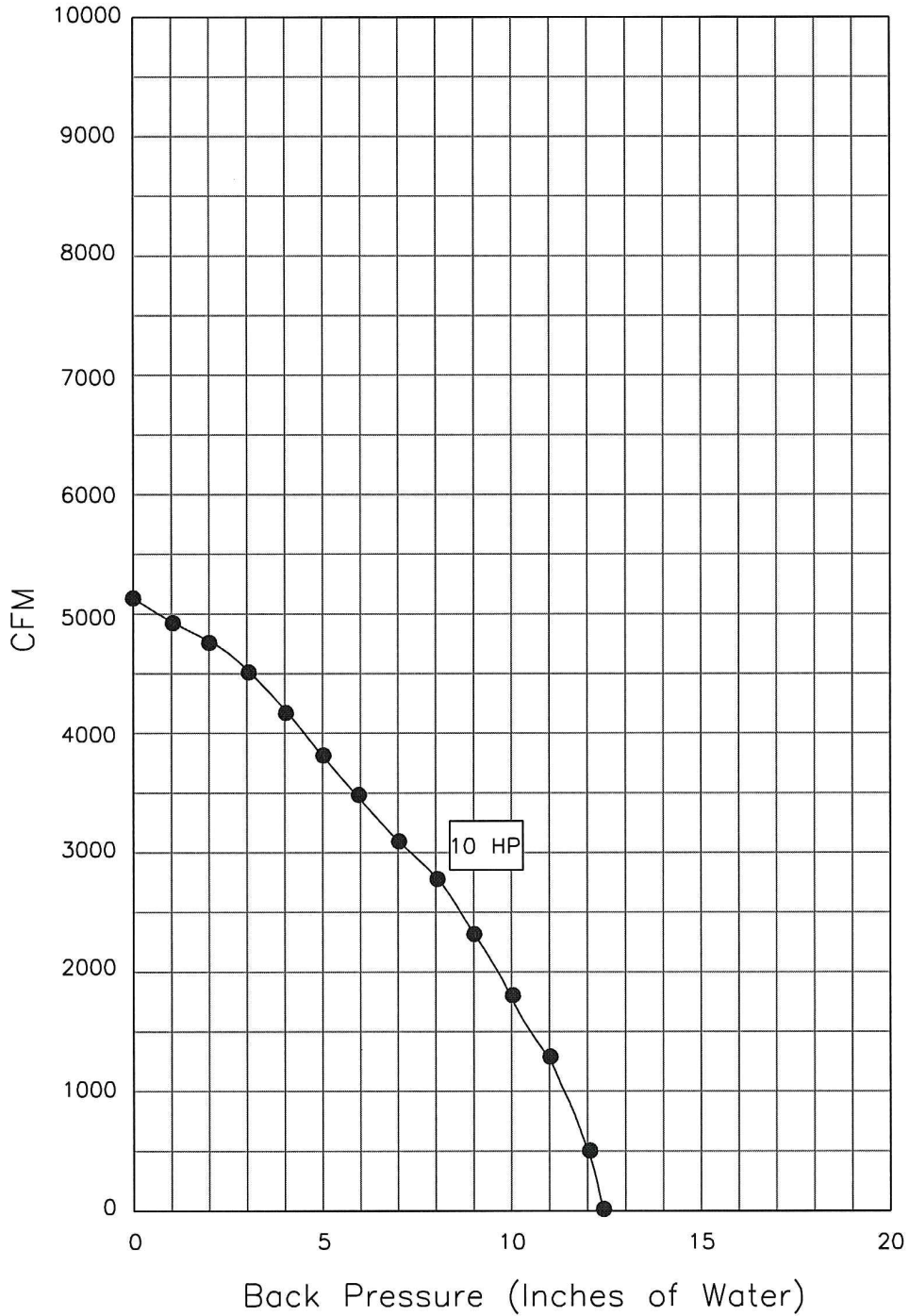
10 H.P. - 1800 RPM ELIMINATOR BLOWER CURVE, 60 HZ.
